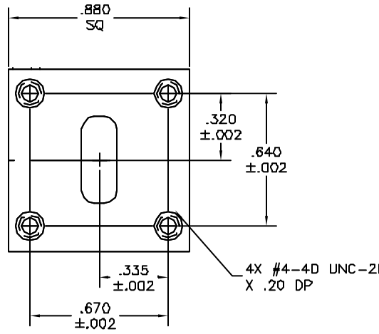
DETAIL A WR-42 WAVEGUIDE
