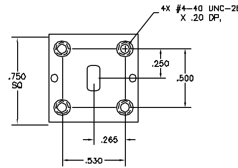
DETAIL A WR-22 WAVEGUIDE
