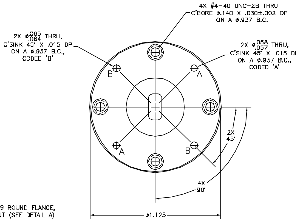
DETAIL A WR-19 WAVEGUIDE
