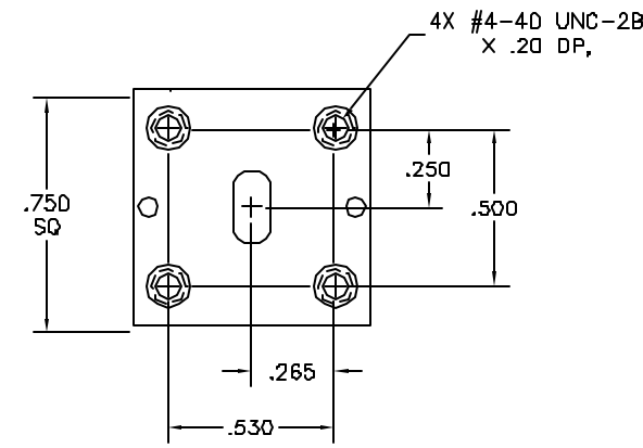
DETAIL A WR-2B WAVEGUIDE
